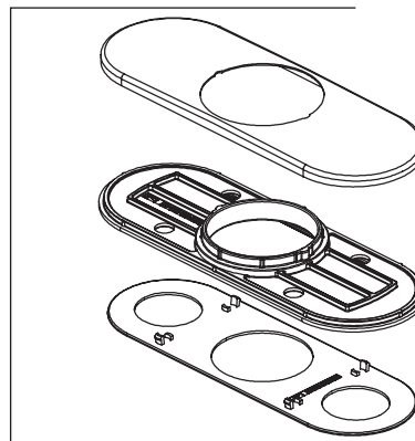
RP103334▲ (Escutcheon optional, included) Escutcheon with Gasket (3 Hole) Chapetón y Empaque (3 agujeros) Boîtier et Joint (3 trous)
